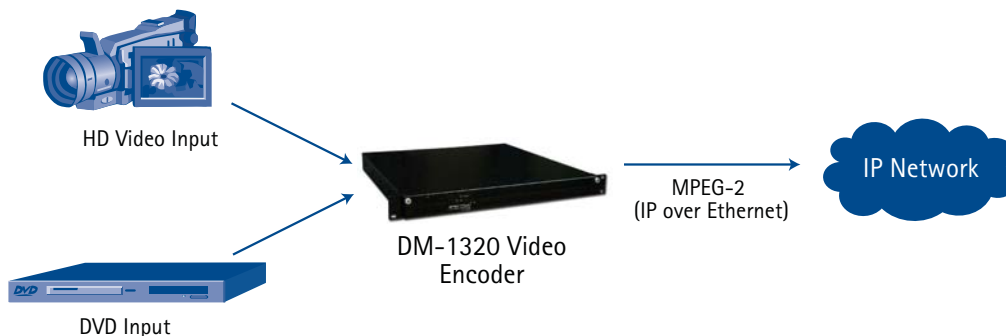
Figure 1. Example Usage for DM-1320 as an Analog HD to MPEG-2 Video Encoder
