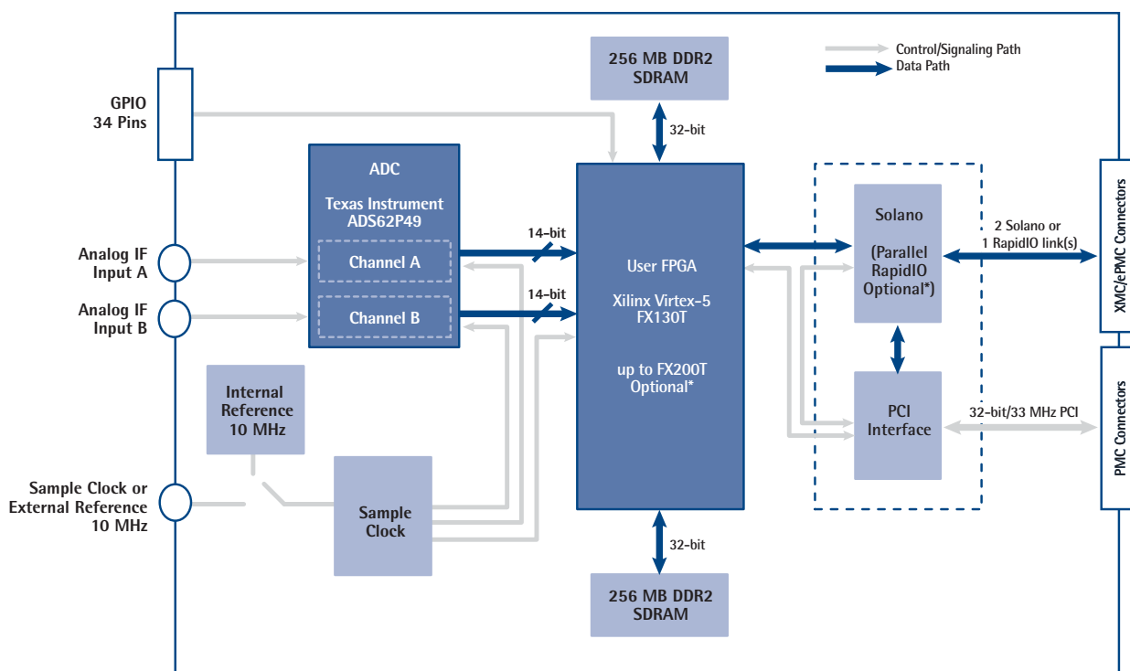
Figure 1. XMC-1131 Block Diagram
