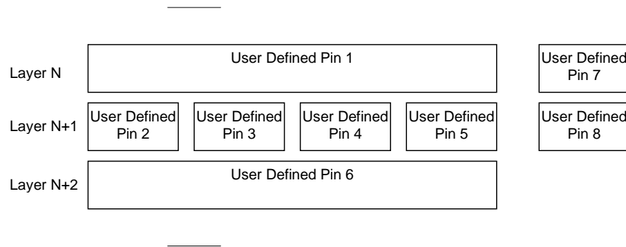
Figure 12 User-Defined Pin PCB Trace Cross Section
