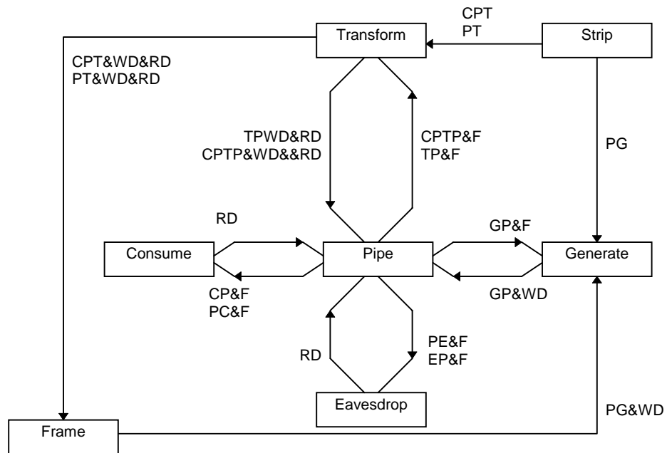
Figure 16 HP BALLISTIC IC State Transition Diagram
