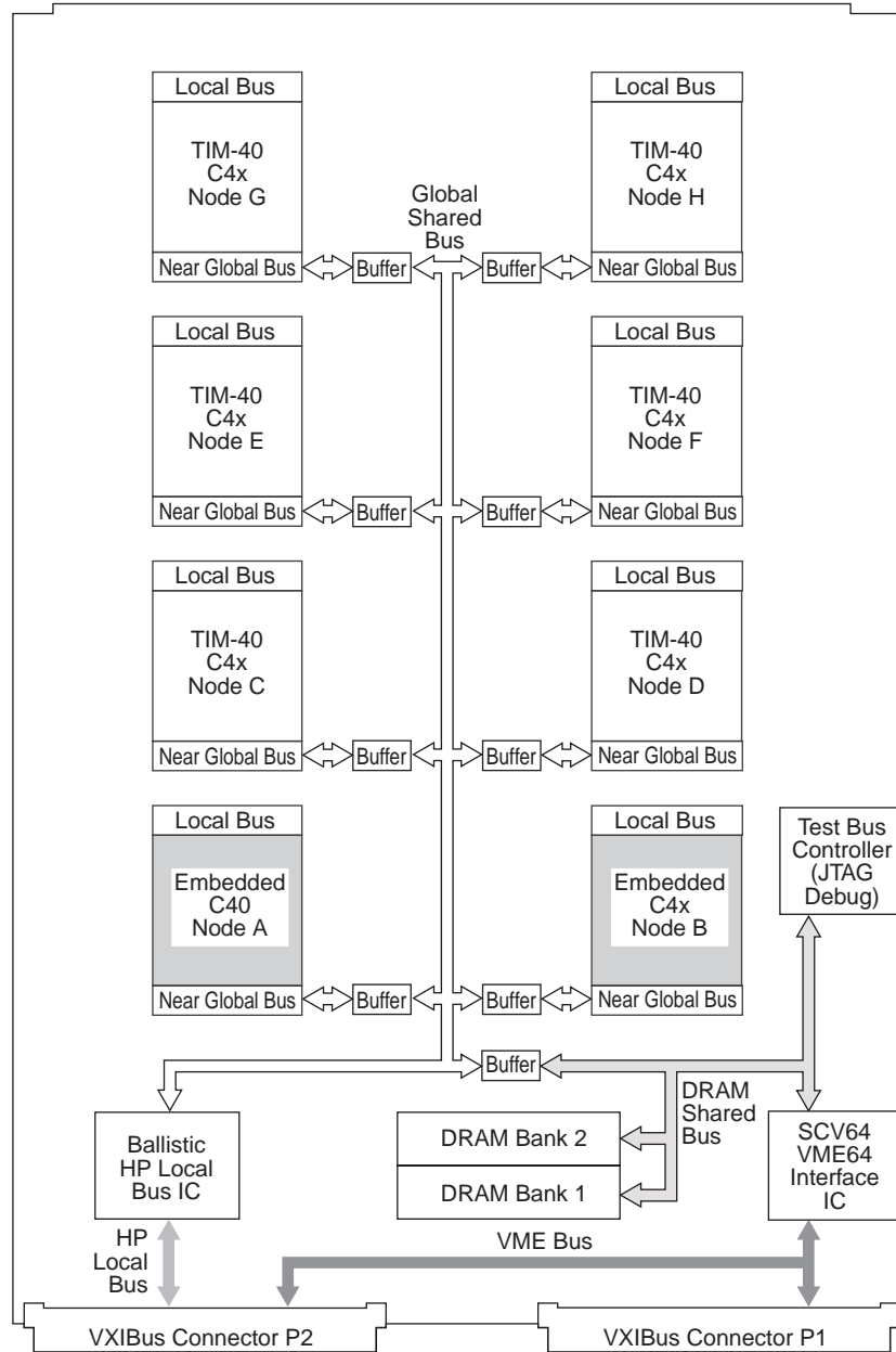
Figure 4 Bus Architecture
