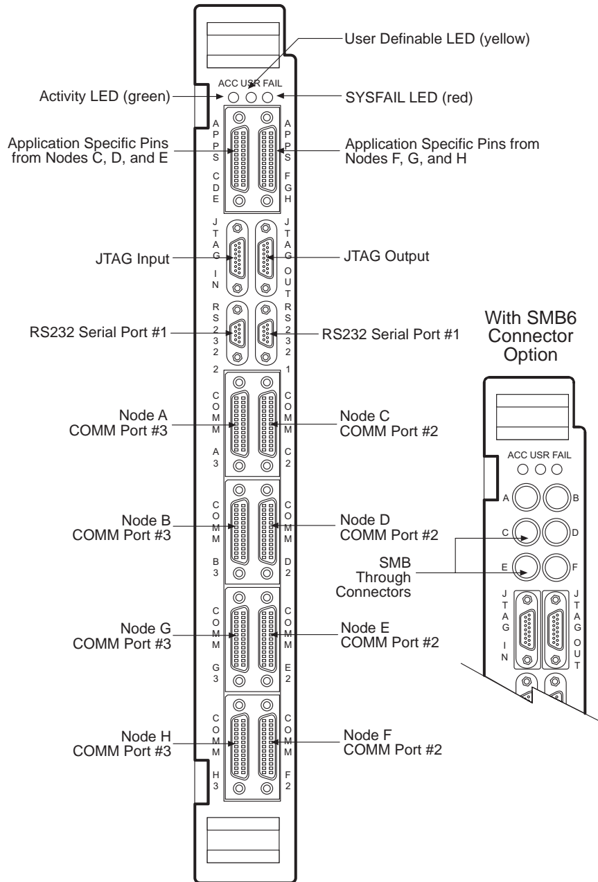
Figure 2 VX8 Front Panel
